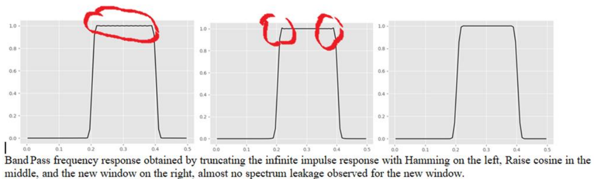
Fig.2. FIR band pass frequency response
