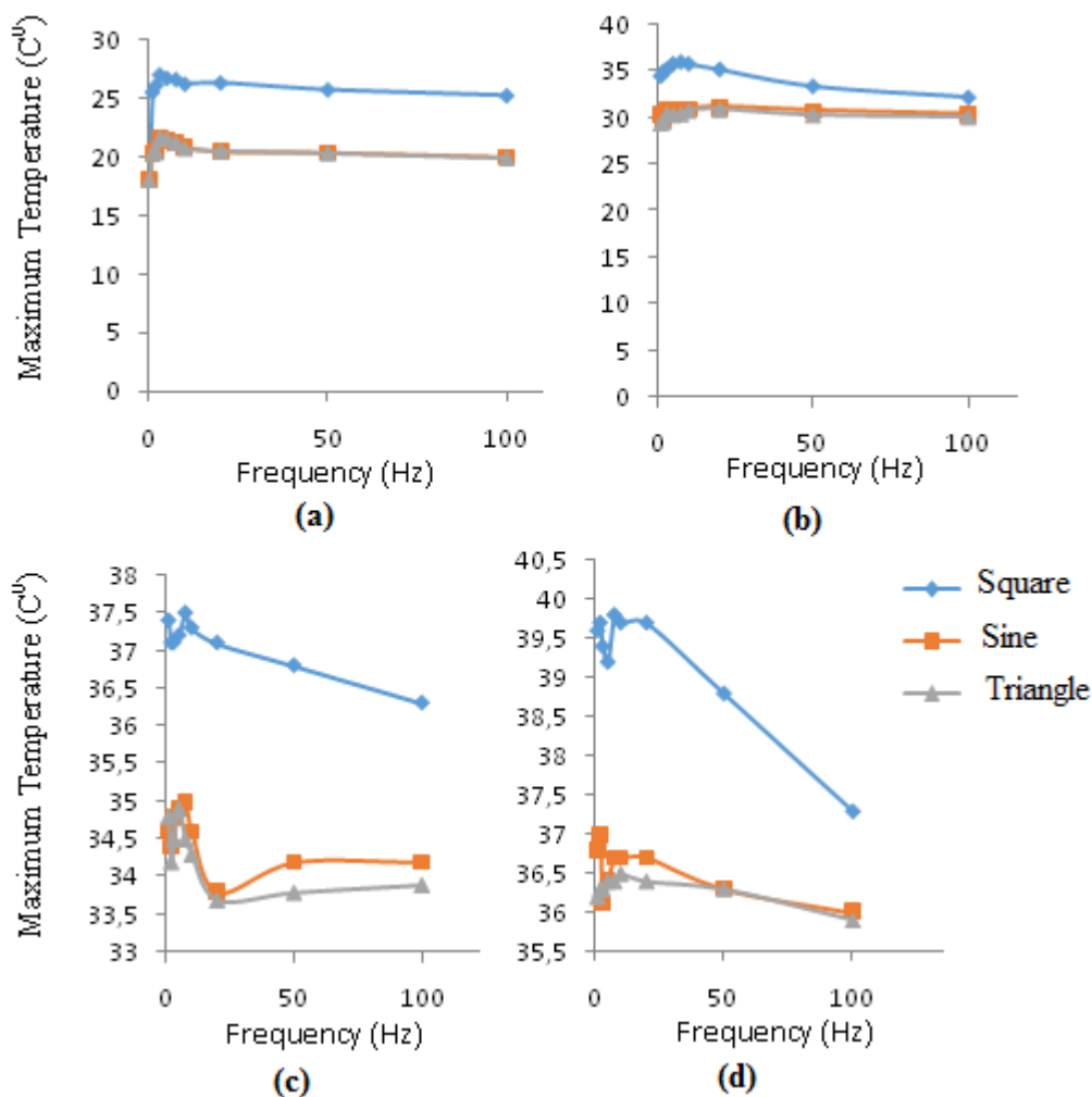
Figure 5. (a) Temperature change graphs on the DEA surface at 18C°, different waveforms, (b) Temperature change graphs on the DEA surface at 25C°, different waveforms, (c) Temperature change graphs on the DEA surface at 29C°, different waveforms, (d) Temperature change graphs on the DEA surface at 32C°, different waveforms.
