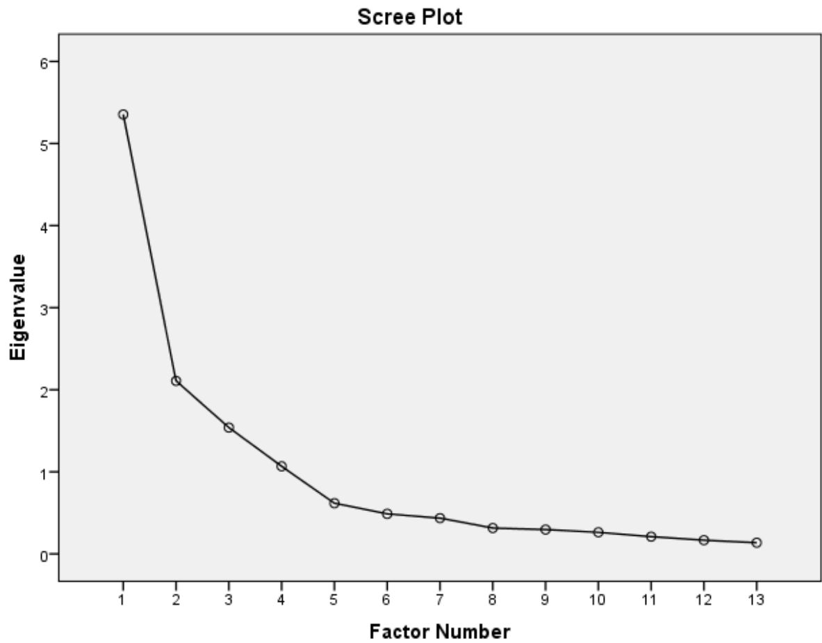
Scree Plot
