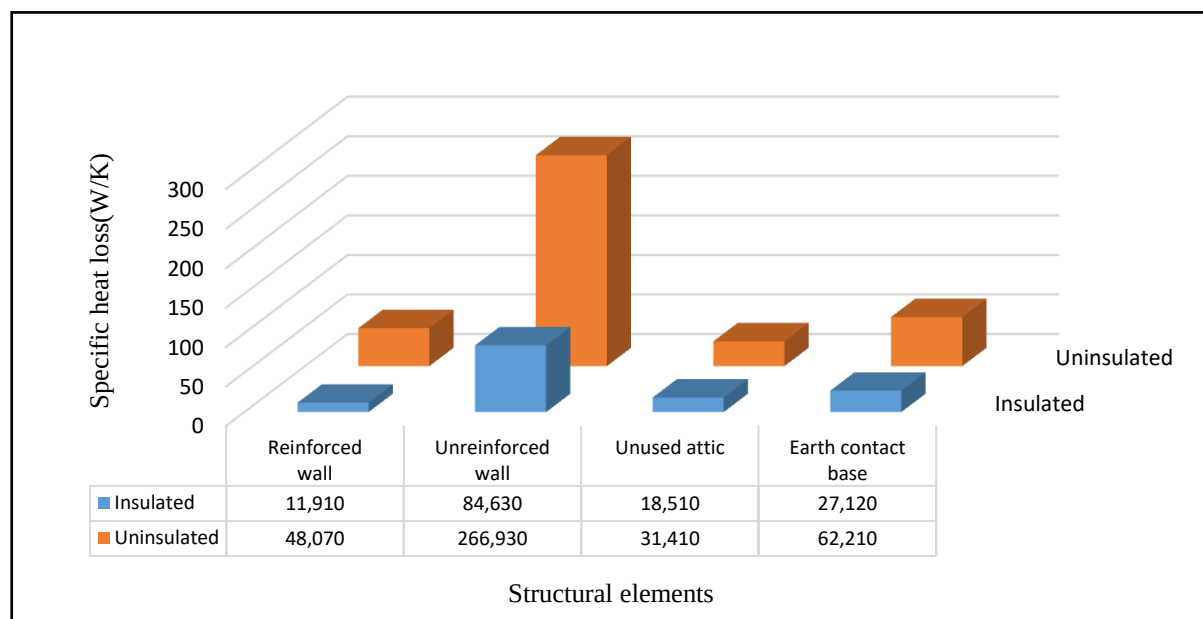
Figure 2. Specific heat loss values of building elements
