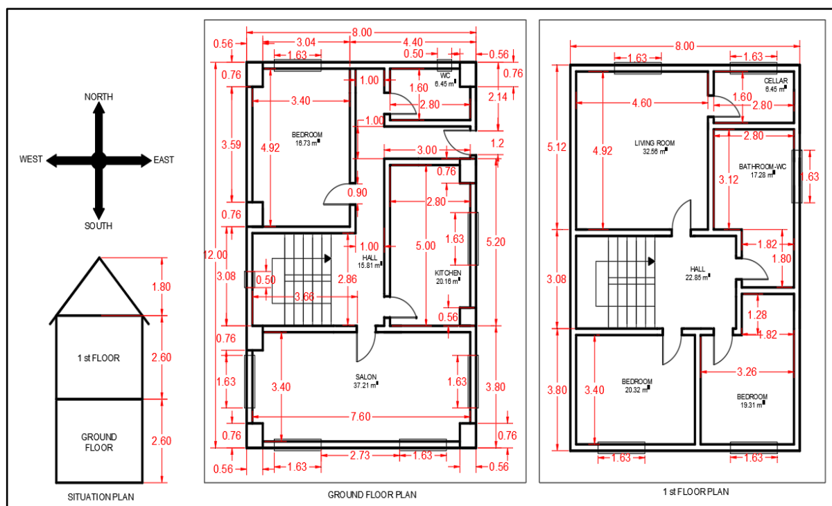
Figure 1. Floor plan of the exemplary architecture
