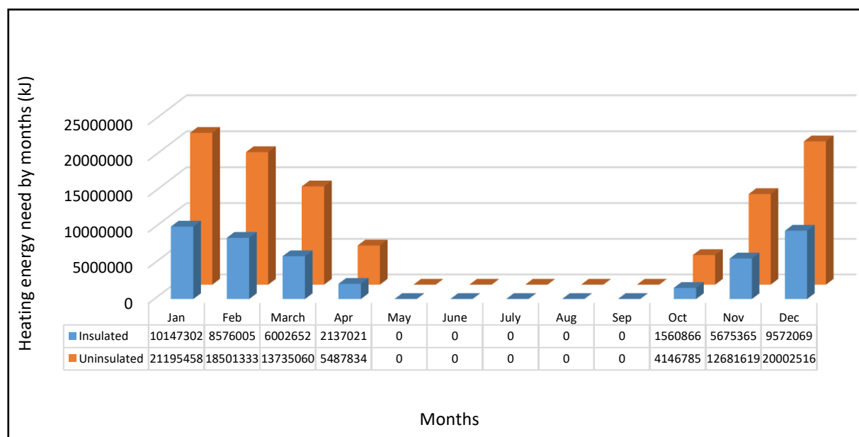
Figure 3. Heating energy need of insulated and uninsulated building by months
