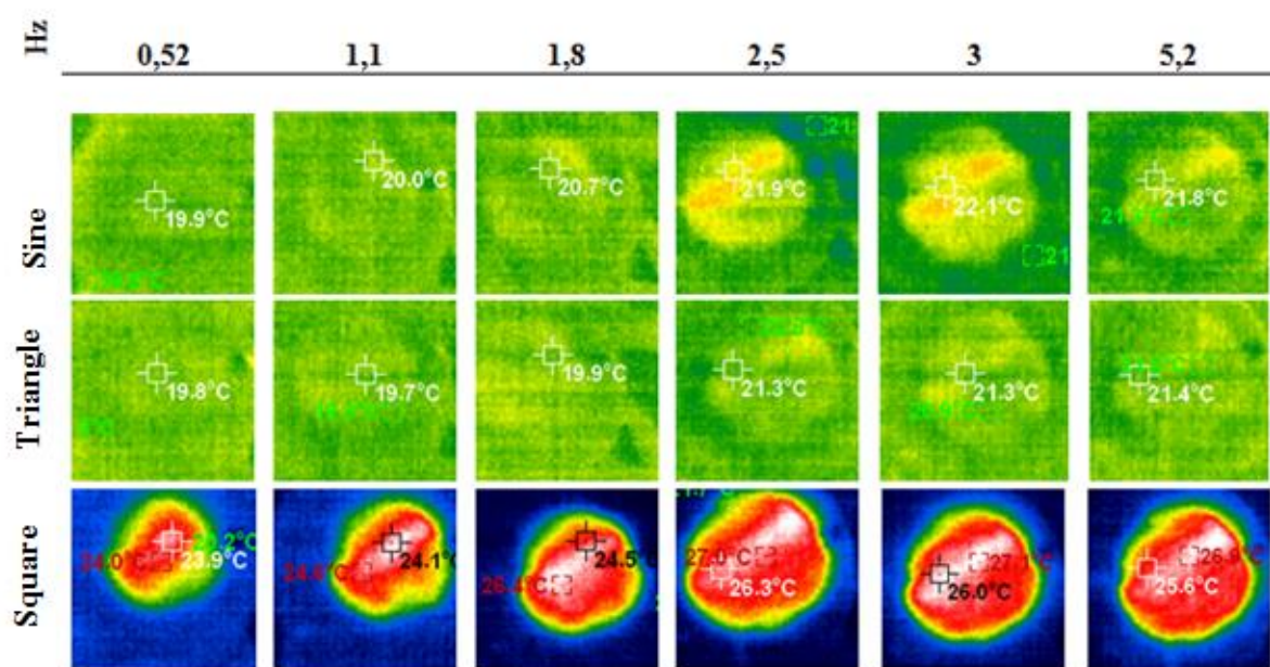
Figure 4. Temperature change thermal imager images in different electrical signals and different frequencies occurring on the DEA surface.
